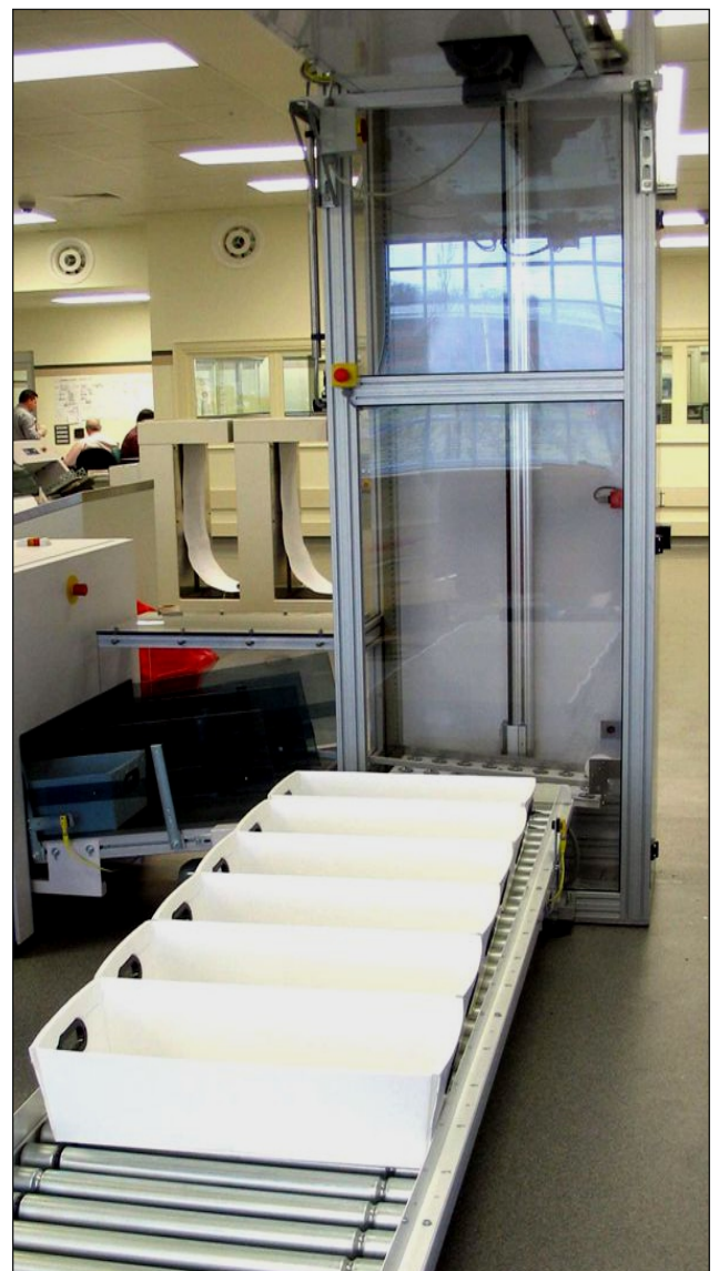
Automatic lift used for transferring tote bins 300mm x 400mm from floor level to overhead roller conveyors.
