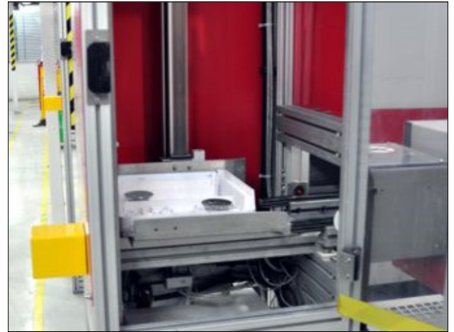
Closeup of lift platform and lower transfer.
