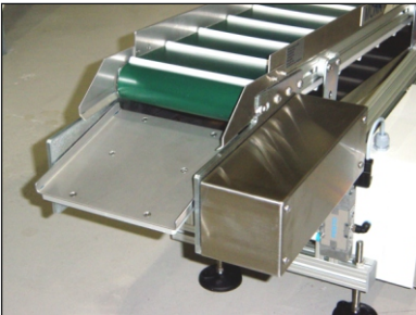
Spreading Discharge Chute
