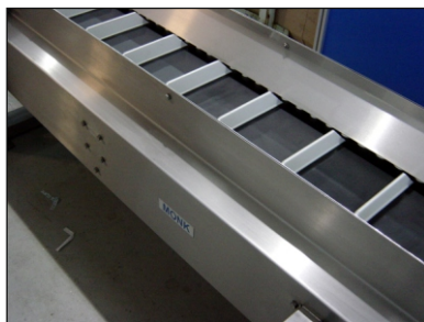
Stainless Steel Conveyor for Dust
