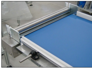
End Rollers
