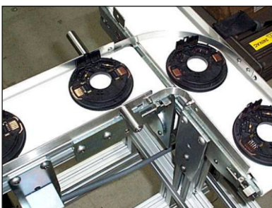
90 Degree Transfers
